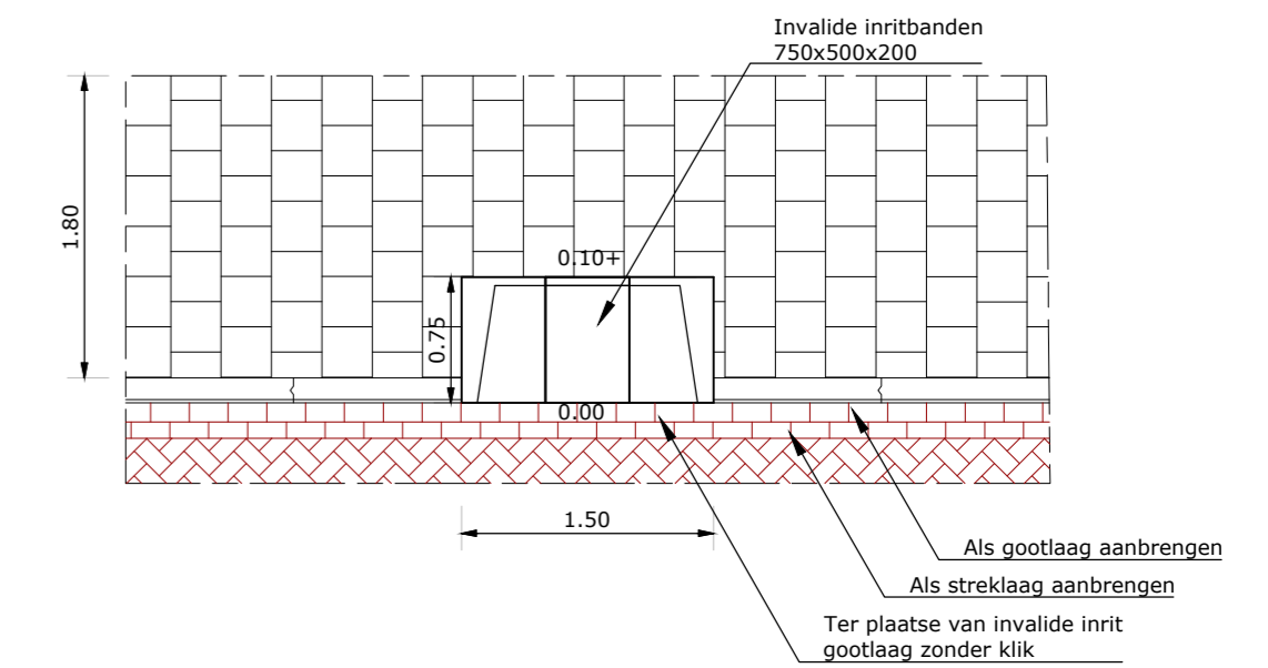
DETAIL INVALIDE INRIT
