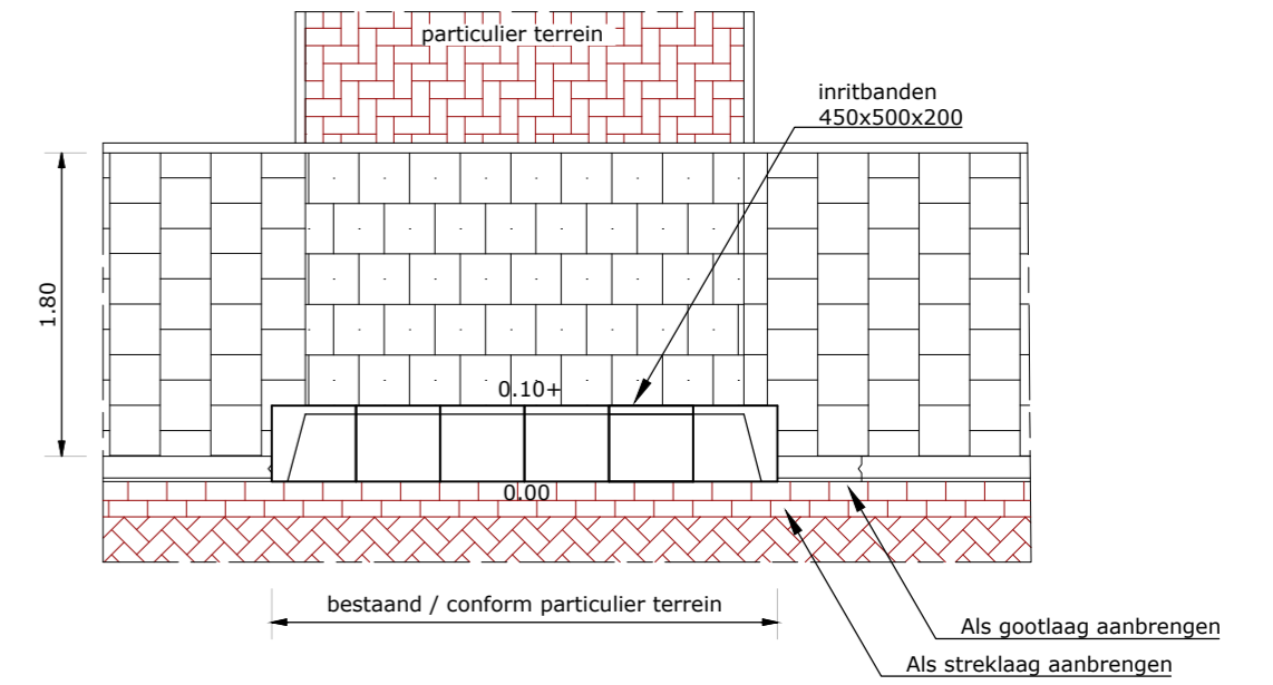
DETAIL PARTICULIERE INRIT
