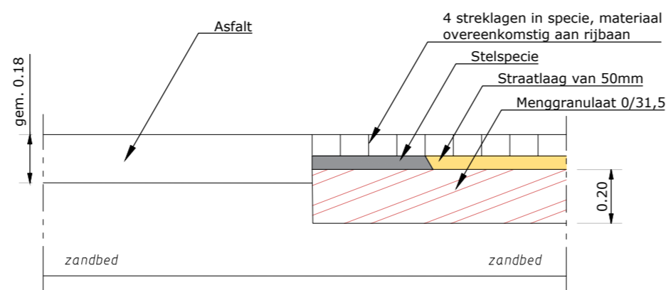
DETAIL OVERGANG ASFALT - ELEMENTEN
